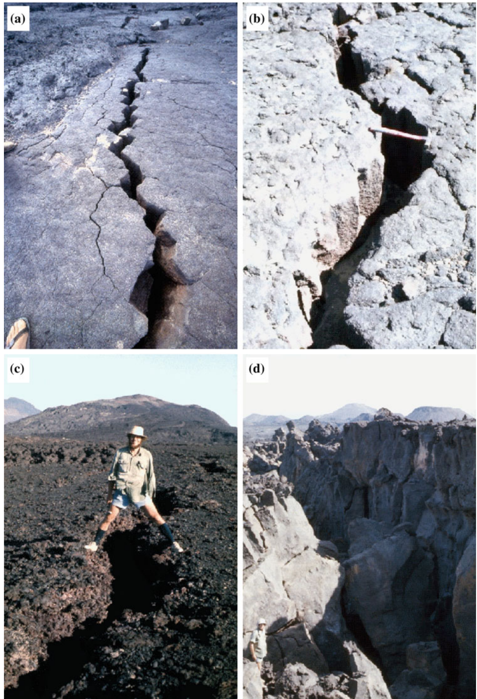
Fig. 5 Open fissures in basalts moving progressively away from the axial neo-volcanic zone in the Ghoubbet–Asal rift. Basalts in a , b display a “polygonal” surface typical of submarine eruptions. c Open fissure; d fissure with vertical offset
